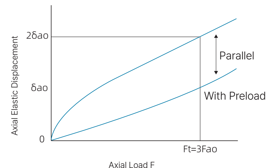
Elastic Displacement Curves of Ball Screw
